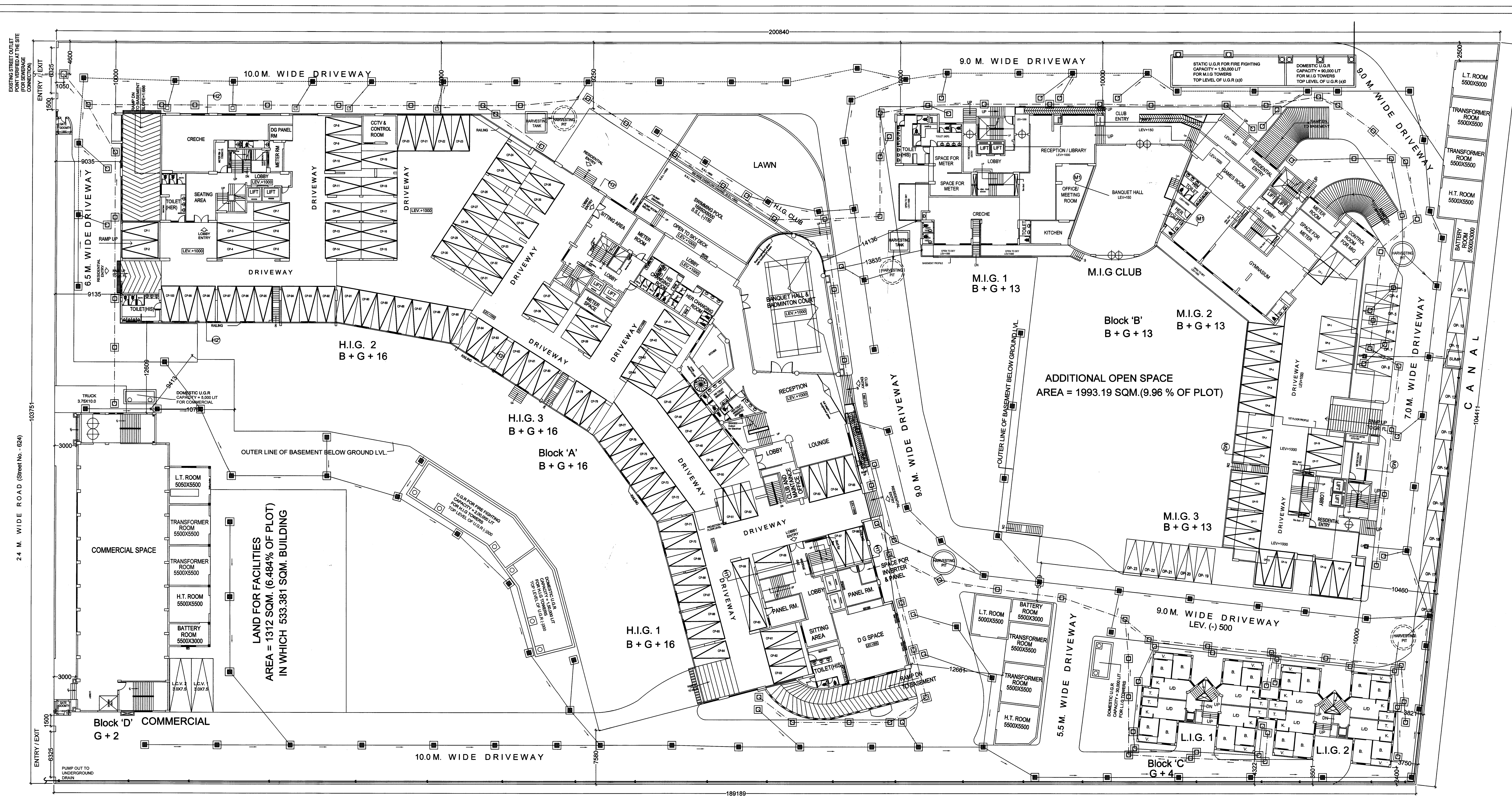
MASTER PLAN SHOWING SEWER & STORM LINE
